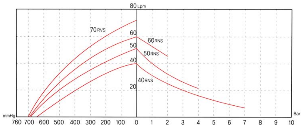
Rocking Piston Pump (Single Head)
